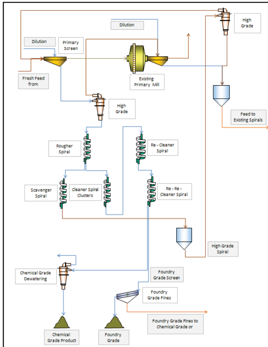
Figure 11.2_4 Foundry Project Simplified Flow Diagram
