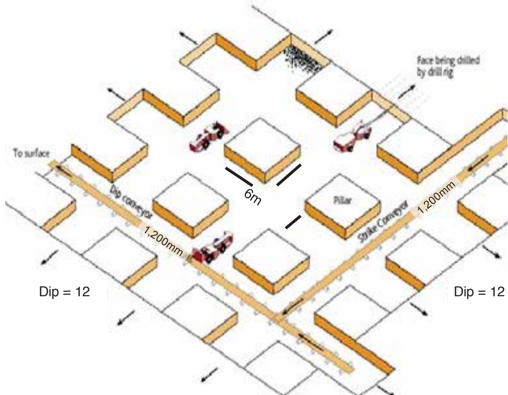
Typical Bord and Pillar Layout
