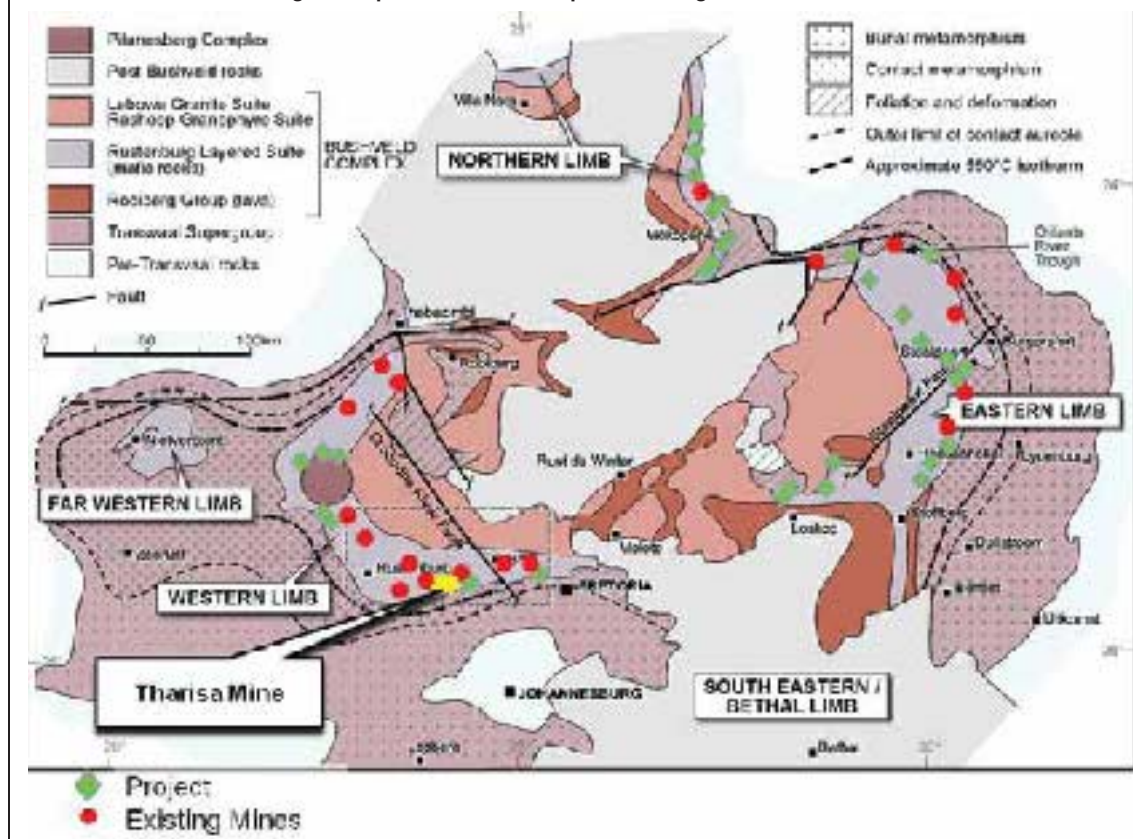
Figure 3.1.2 Generalised Geological Map of Bushveld Complex Showing the Location of the Tharisa Mine
