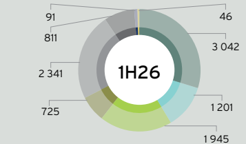
Value distribution (Rm)
