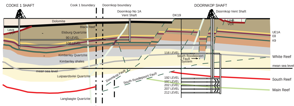
Cooke 1/Doornkop geological section looking west
