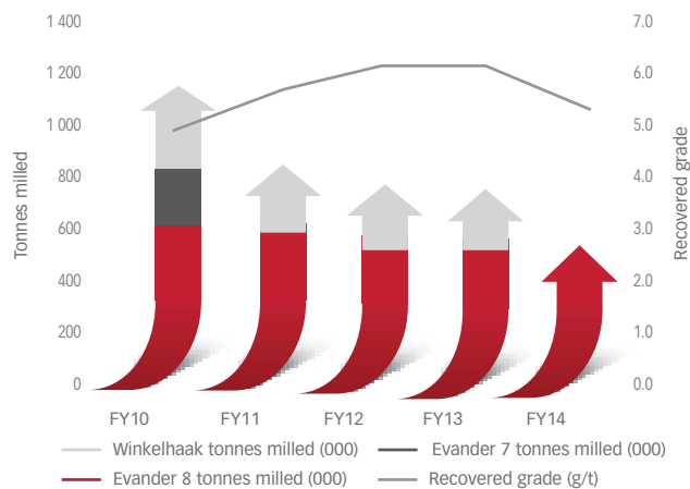
Evander: Five-year production profile
