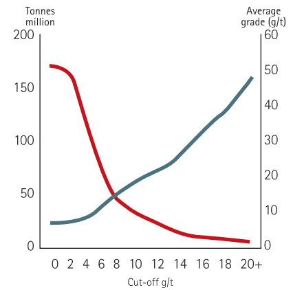
Orkney grade tonnage curve - Indicated
