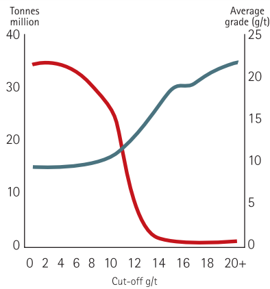
Elandsdraal grade tonnage curve - Indicated
