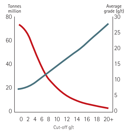
Freegold grade tonnage curve - Measured
