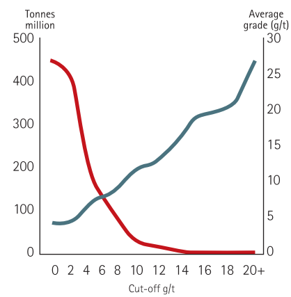
Freegold grade tonnage curve - Inferred
