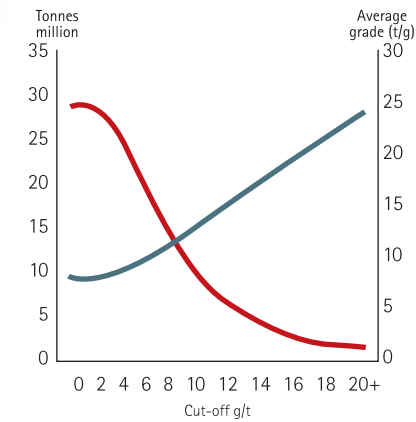
Elandsdraal grade tonnage curve - Measured
