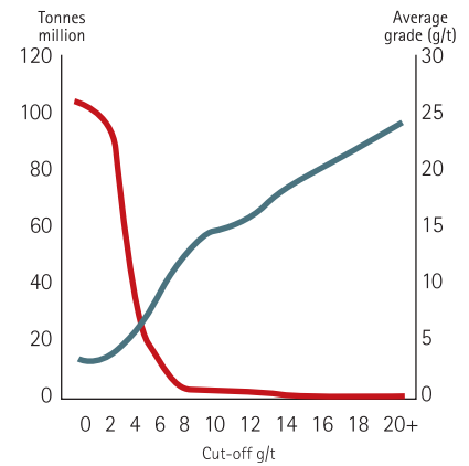
Orkney grade tonnage curve - Inferred
