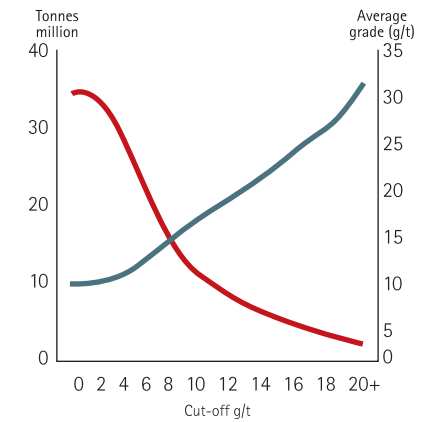
Orkney grade tonnage curve - Measured
