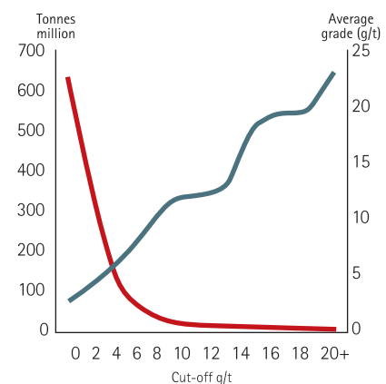
Randfontein grade tonnage curve – Inferred
