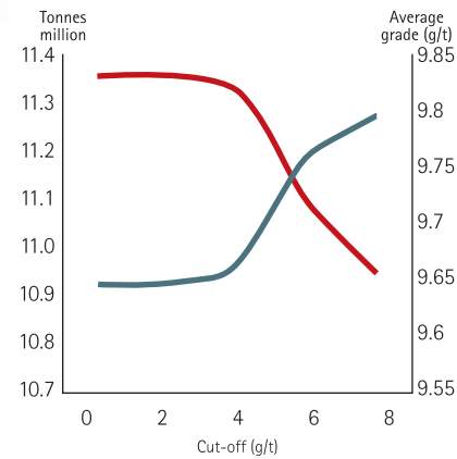
Elandsdraal grade tonnage curve - Inferred
