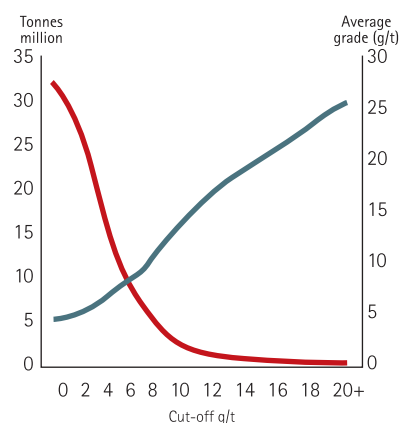
Welkom grade tonnage curve – Measured
