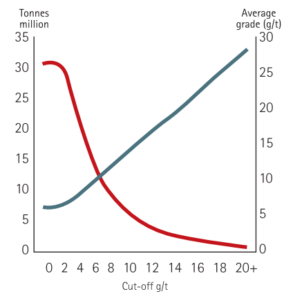
Evander grade tonnage curve - Measured
