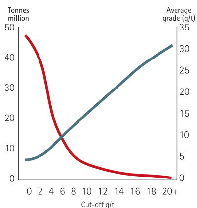
Randfontein grade tonnage curve – Measured
