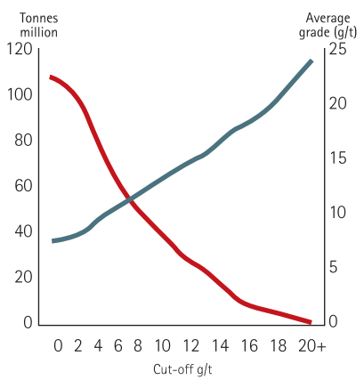
Freegold grade tonnage curve - Indicated
