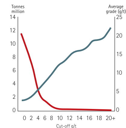
Welkom grade tonnage curve – Inferred
