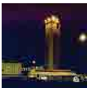
Driefontein gold mine, South Africa
