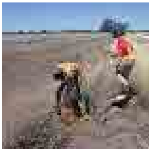
Exploration geochemical sampling, Central Victoria Project, Australia
