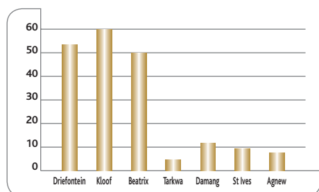
Electricity used per ton gold produced (GWh per ton gold produced)
